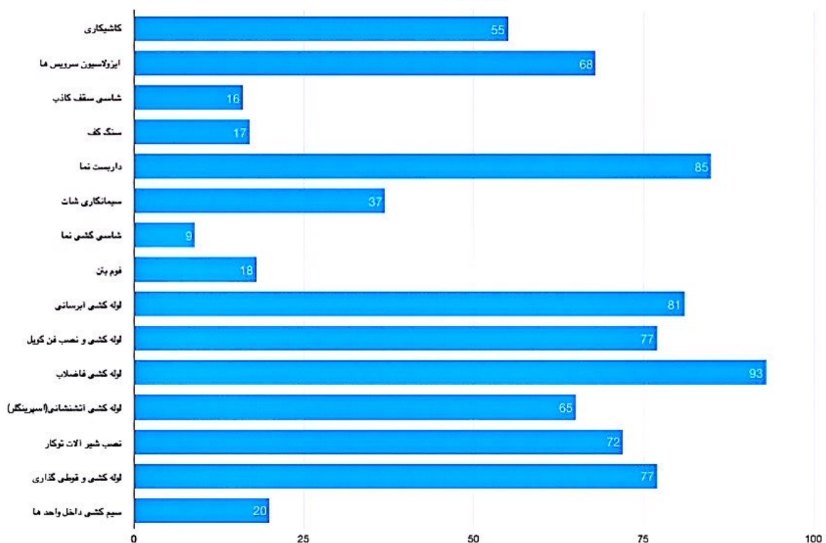
Bar Chart
