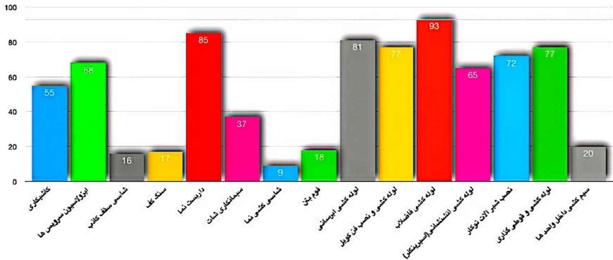
Column Chart
